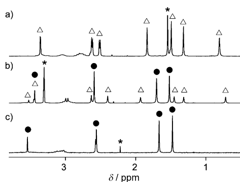
Figure 3. a–c) 1 H NMR spectra of 3 ·( \text{BF}_4 ) 2 in \text{CD}_2\text{Cl}_2 (a), \text{CD}_3\text{OD} (b), and \text{D}_2\text{O} (c). The methyl signals of 3 2+ and 4 + are represented by Δ and ●, respectively. δ Values are given relative to tetramethylsilane (TMS; a, b) or sodium 4,4'-dimethyl-4-silapentane-1-sulfonate (DSS; c).
